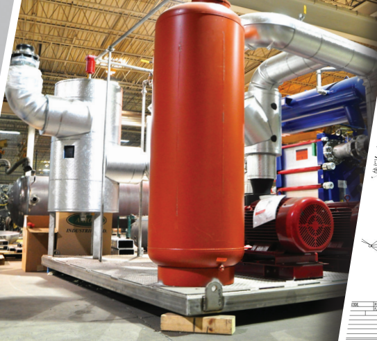
Skidded Chiller Package With Glycol Pumping System
