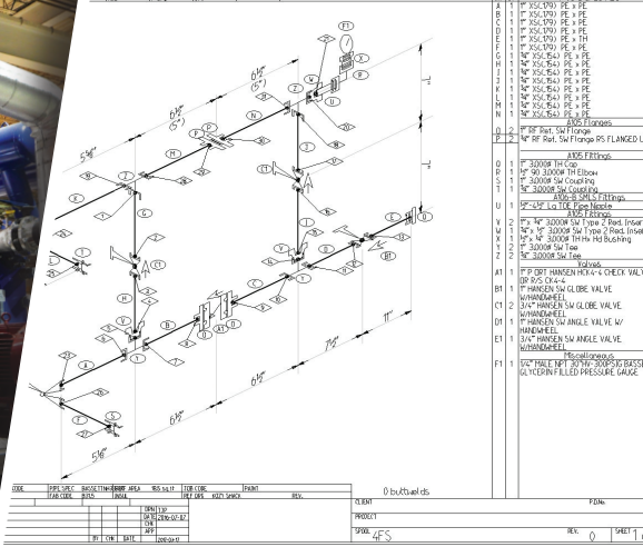
Piping Isometric With Weld & Material Map
